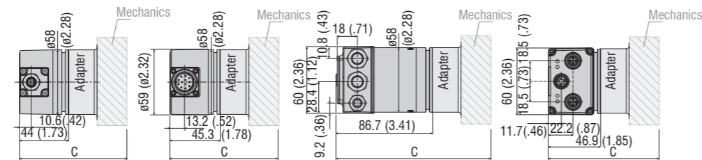
Dimensional drawing WDS- ... - P200 - CR - HTL/TTL Dimensional drawing WDS- ... - P200 - SR - SSI Dimensional drawing WDS- ... - P200 - BH - CO/PB Dimensional drawing WDS- ... - P200 - BH - PN/ENIP/CAT
