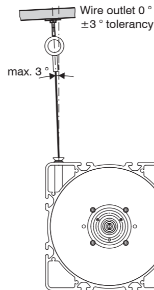
Attachment and maximum diagonal pull of the measuring wire
