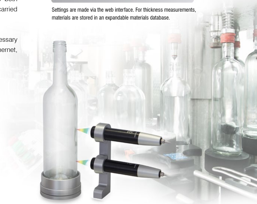
Two sensors can be directly connected to a confocal IFC2422 controller.
