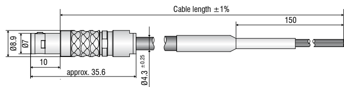
SCAC3/5 Signal output cable (Art.-no. 2902112)
