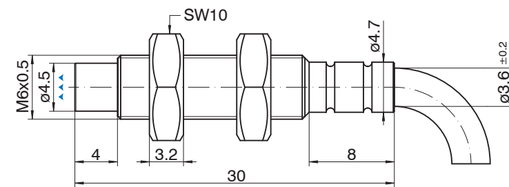
Fig. 5 ES-U1-C-CAx, dimensions in mm (not to scale)
